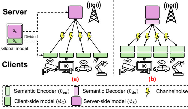
Fig. 1. Overall framework of the proposed CA-SSFL scheme. (a) The global model is divided into client-side and server-side sub-models for split federated learning. (b) The client-side semantic encoder compresses smashed data before wireless transmission, and the server-side semantic decoder restores the received latent representation for downstream prediction.
